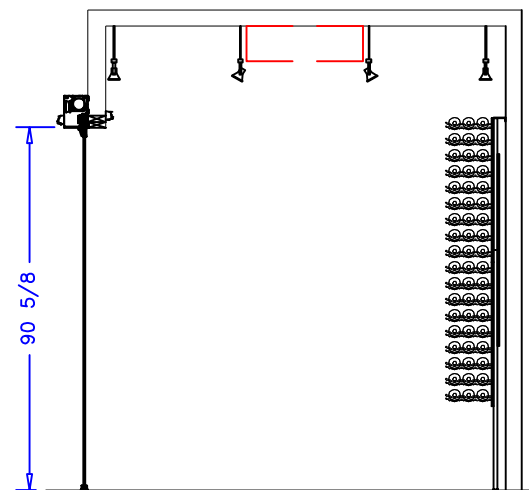
DOOR (C) SECTION
